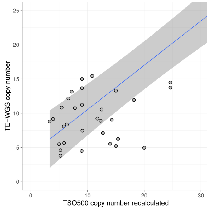
S1 Fig. Zoomed-in view of the Fig. 3C, showing concordance in gene amplification copy number between TruSight Oncology 500 (TSO500) and TruSight Oncology 500 (TE-WGS), after adjusting for tumor purity by TE-WGS.
