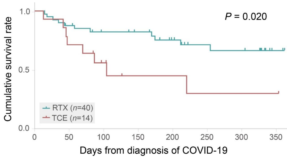
S6 Fig. Comparison of overall survival between the T-cell engager (TCE) and rituximab (RTX) groups. COVID-19, coronavirus disease 2019.
