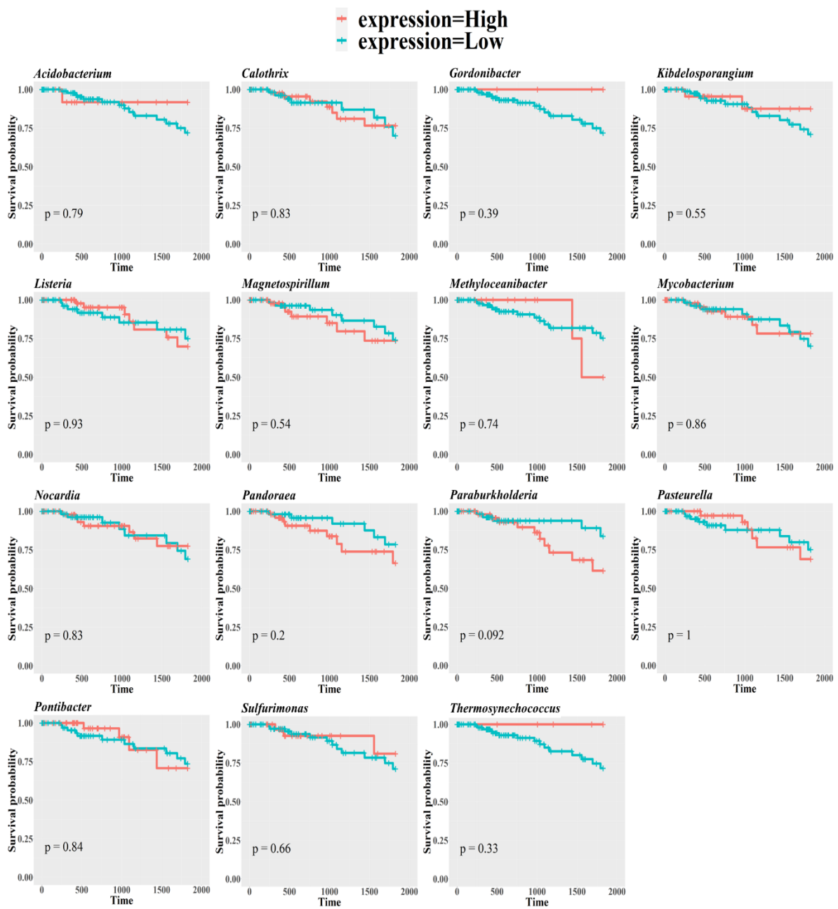
S6 Fig. The Kaplan-Meier curve of the 5-year survival analysis based on triple-negative breast cancer patient microbiome count data from the Cancer Genome Atlas. The microbiome selected was not affected by outliers.
