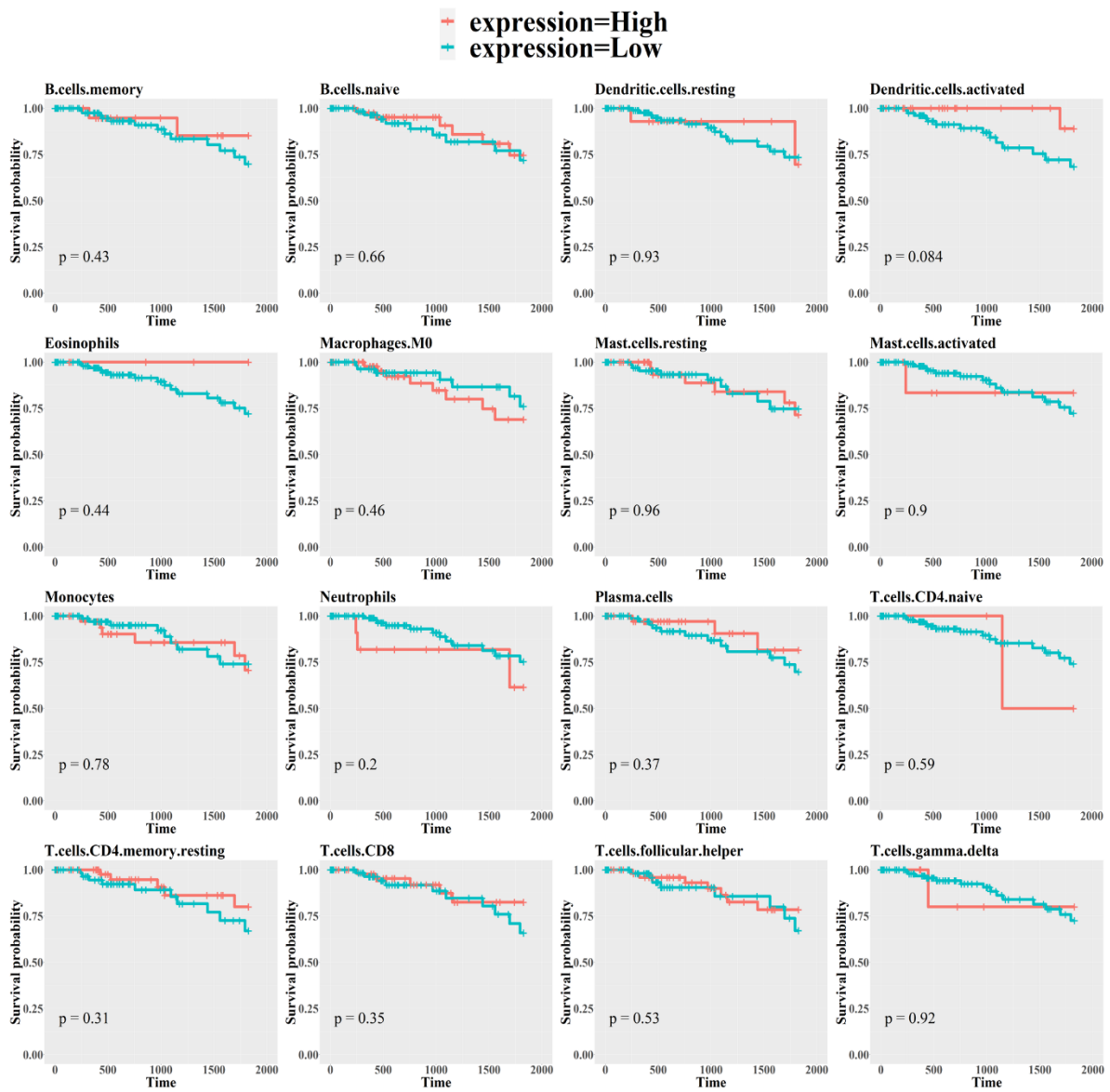
S5 Fig. The Kaplan-Meier curve of 5-year survival analysis based on triple-negative breast cancer patient immune cell fraction data from The Cancer Genome Atlas (TCGA).
