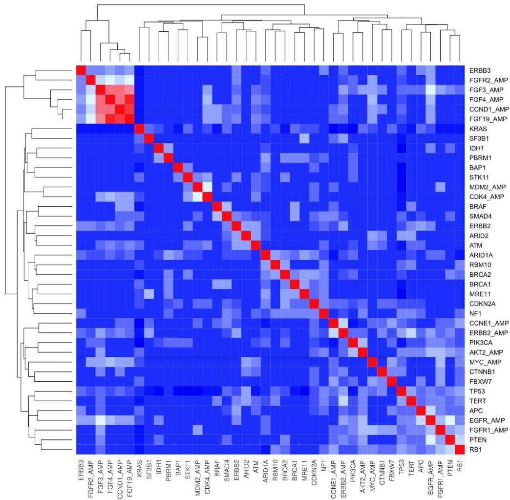
S3 Fig. Clustered matrix of the correlation with co-occurrence of frequently mutated genes in biliary tract cancer. Correlation with the centroid linkage approach was used to identify clustered matrix.
