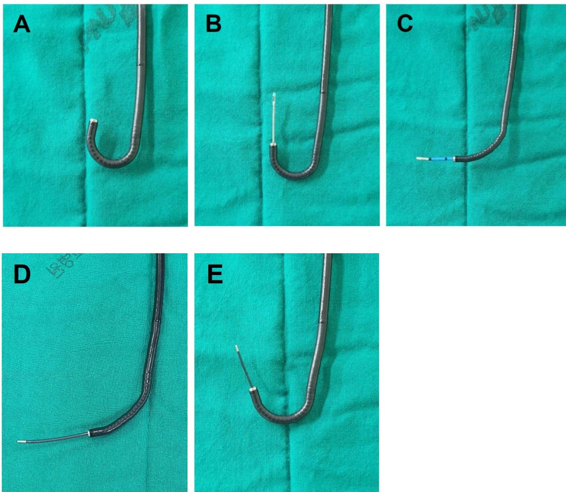
S1 Fig. Bending angles of 4.0-mm diameter thin bronchoscope with 2.0-mm diameter channel. (A) Maximal upward manipulation of the thin bronchoscope without placing anything in the bronchoscopy channel. (B) Maximal upward manipulation of the thin bronchoscope with radial probe endobronchial ultrasound in the bronchoscopy channel. (C) Maximal upward manipulation of the thin bronchoscope with a 1.9-mm diameter reusable cryoprobe in the bronchoscopy channel. (D) Maximal upward manipulation of the thin bronchoscope with a 1.7-mm diameter disposable cryoprobe in the bronchoscopy channel. (E) Maximal upward manipulation of the thin bronchoscope with a 1.1-mm diameter disposable cryoprobe in the bronchoscopy channel.
