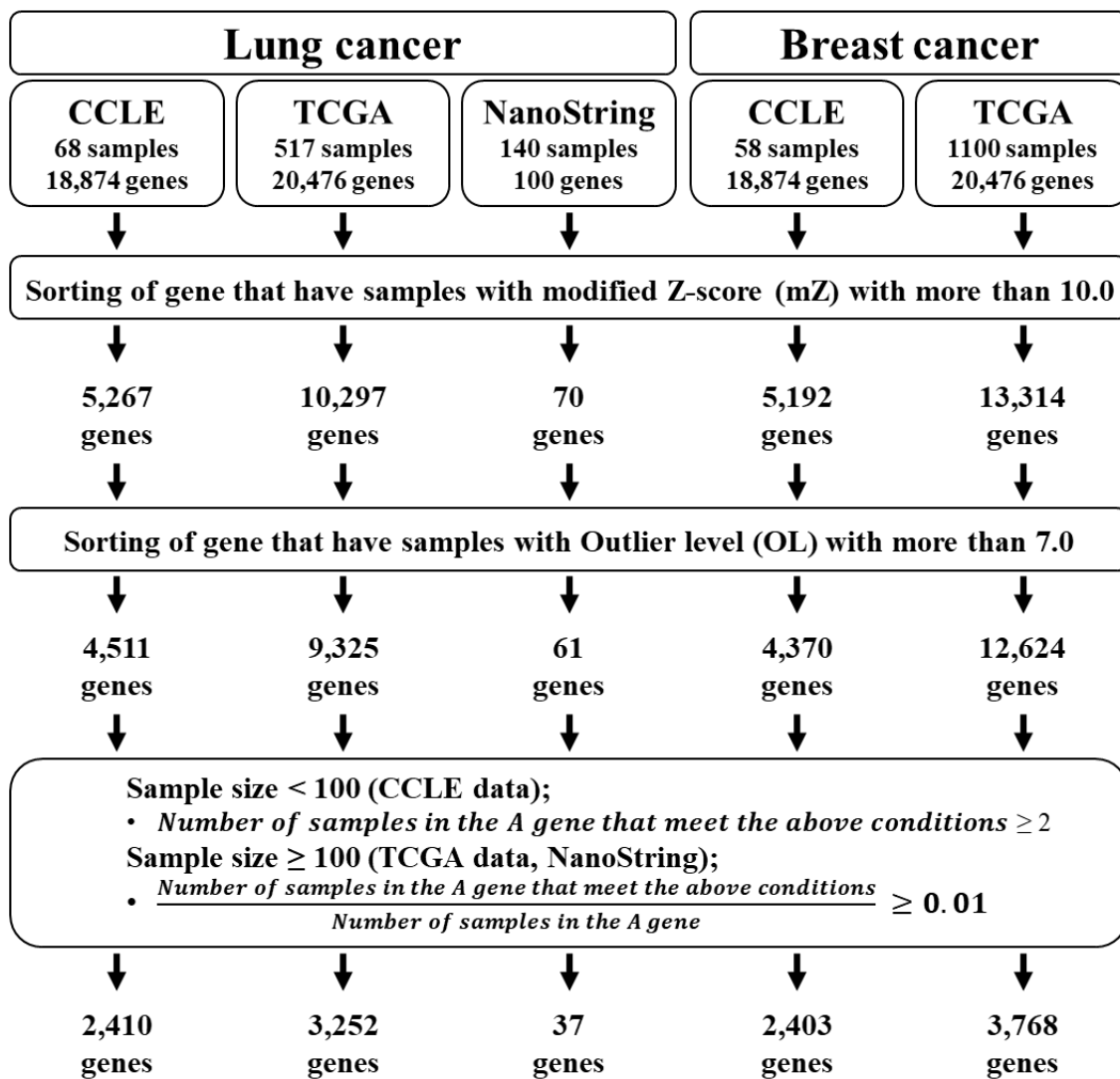
S1 Fig. The scheme of a modified Tukey's Fences method. CCLE, Cancer Cell Line Encyclopedia; TCGA, The Cancer Genome Atlas.
