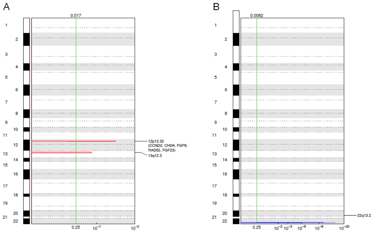
S20 Fig. GISTIC. (A) Significantly amplified region in colorectal cancer. (B) Significantly deleted region in colorectal cancer.
