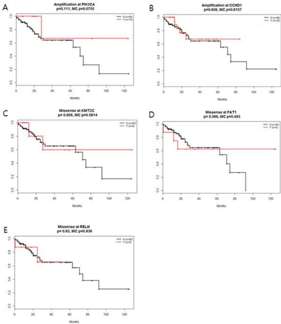
S6 Fig. Kaplan-Meier curves showing the association of highly frequent genetic alterations (> 10%) and overall survival in patients. (A) PIK3CA amplification. (B) CCND1 amplification. (C) KMT2C missense mutation. (D) FAT1 missense mutation. (E) RELN missense mutation.
