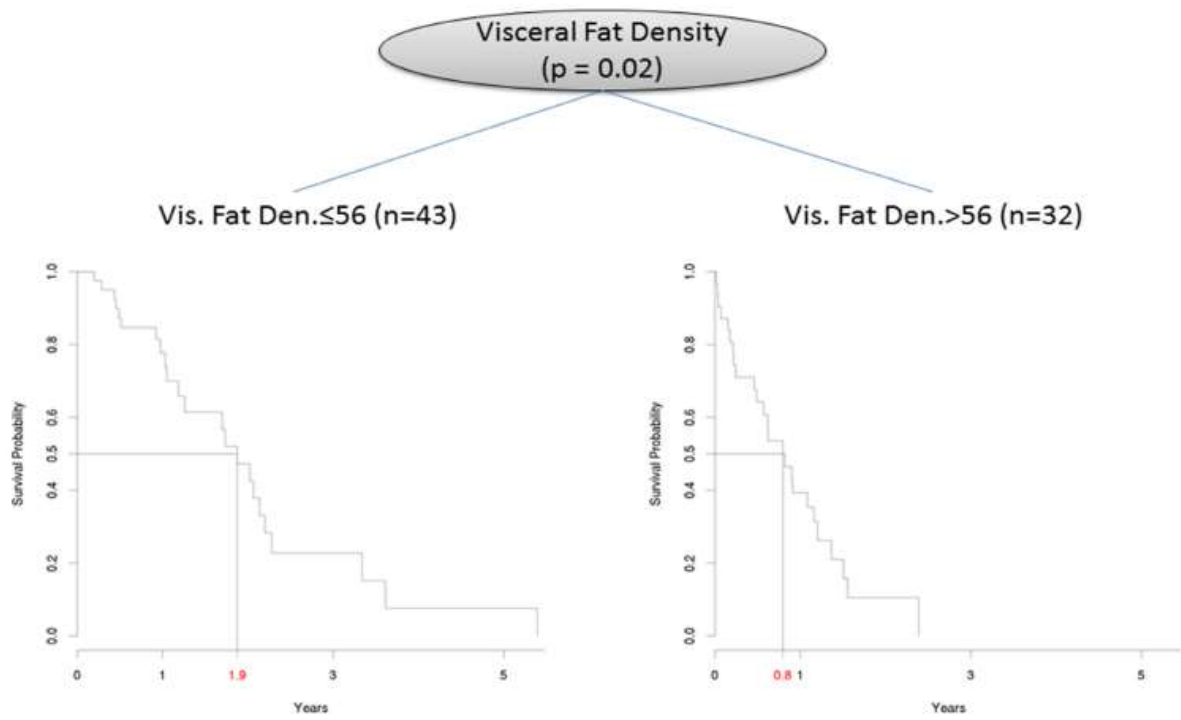
S3 Fig. Conditional inference tree schema.
