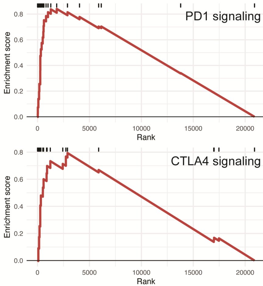
S13 Fig. Get Set Enrichment Analysis. Upregulation of the programmed death 1 (PD-1) signaling pathway (upper) and CTLA-4 signaling pathway (lower) in programmed death-ligand 1 (PD-L1)-positive bladder cancers compared to PD-L1-negative bladder cancer.
